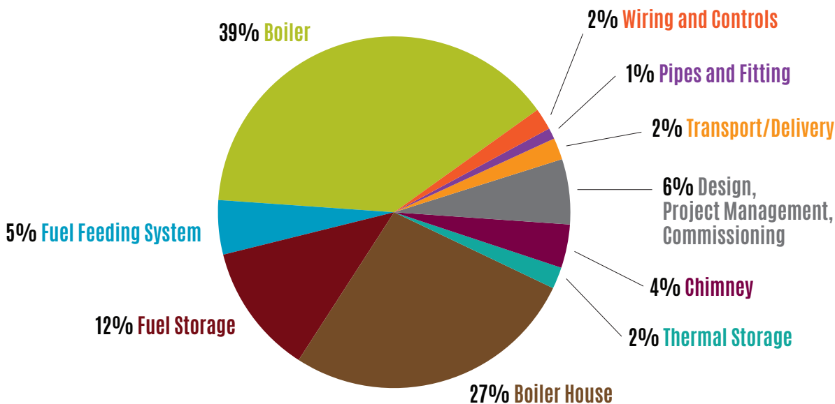
FIGURE 17: Example of capital cost breakdown where a new boiler house is required Based on BERCC analysis of project costs
