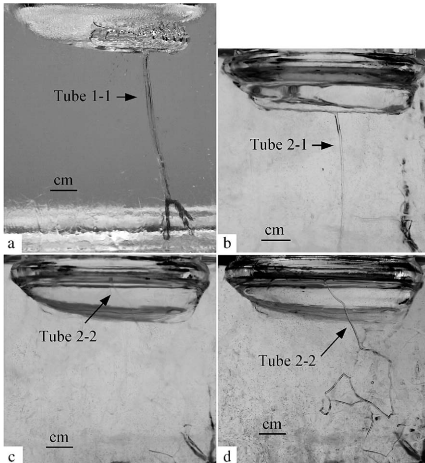
Fig. 2. Melt pools and fuel tubes in experiments 1 and 2. (a) Fuel tube 1-1 in block 1, 106 h into experiment 1; (b) fuel tube 2-1 in block 2, 24 h into experiment 2; (c) first visible movement of fuel in tube 2-2, 32 h into experiment 2; (d) tube 2-2 three minutes after first visible fuel movement shown in Fig. 2c.
